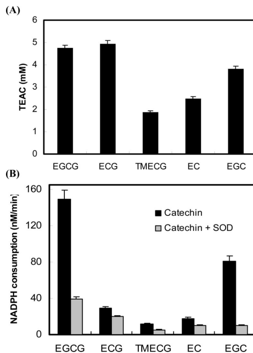
Figure 3. (A) Antioxidant activity of TMECG and tea catechins expressed as TEAC and determined as detailed in the Experimental Section. (B) Prooxidant activity of TMECG and tea catechins determined by their NADPH oxidation capacity in the absence or the presence of SOD. The rate of the oxidation of NADPH (0.1 mM) was calculated in the presence of 50 \mu M catechins in sodium phosphate buffer at pH 7.4, 37 ^{\circ} C. The effect of SOD on catechin-dependent NADPH oxidation was studied in the presence of 10 \mu g/mL of enzyme.
