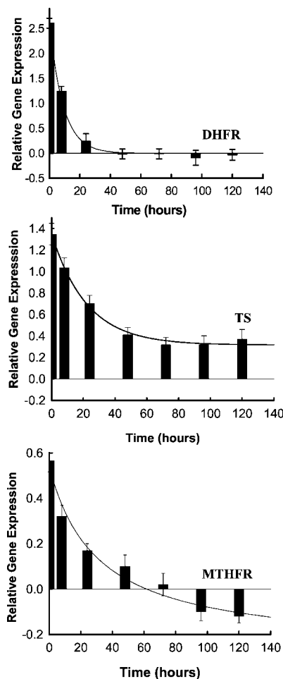
Figure 5. Time-dependent expression of DHFR, TS, and MTHFR in SkMel-28 cells treated with 20 \mu M TMECG. Data were obtained by real time PCR and compared with the relative expression of DHFR, TS, and MTHFR in HeM cells (zero relative gene expression). Zero time represents the level of DHFR in untreated SkMel-28 cells. Differences between times were statistically significant ( P < 0.025 ).
