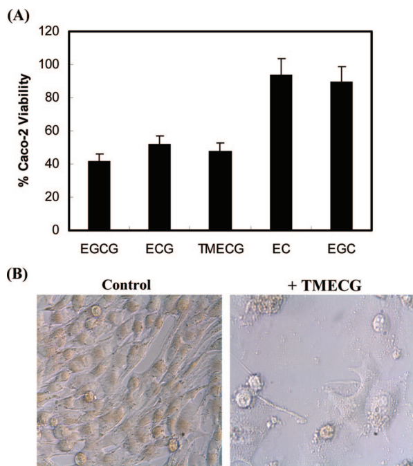
Figure 2. (A) Caco-2 viability after treatments with TMECG and tea catechins and with respect to a control experiment (100% viability) with no compound added. Cells were treated for 6 days with 25 \mu M of each compound. The values presented are the mean percentage determined from three independent experiments \pm SD. (B) Morphological aspect (magnification, 800 \times ) of untreated SkMel-28 cells (control) compared with those subject to 6-days of treatments with 20 \mu M TMECG.
