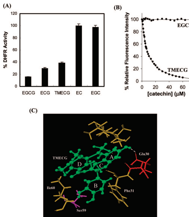
Figure 4. (A) Relative human DHFR inhibition by TMECG and tea catechins (all compounds at 100 \mu\text{M} ) with respect to a control experiment with no compound added. Each bar represents the mean of five separate experiments. (B) Titration fluorescence experiments for the binding of TMECG and EGC to human DHFR. The points are experimental (after correction for enzyme dilution), and the lines are best-fit theoretical curves. The enzyme concentration was 0.1 \mu\text{M} . (C) View of TMECG modeled into the folate-binding site of human DHFR. Atoms of the TMECG ligand are colored green. Four different ligands from human and chicken DHFR crystal structures were used to define a binding envelope. These were placed in a common orientation by superimposing backbone atoms from a common set of protein residues located around the ligands. Ligands from the following PDB structure files were used: 1DR1 (biopterin), 1S3V (TQD), 1S3W, and 1DLR.
