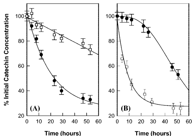
Figure 1. (A) Stability of ECG (●) and TMECG (□) in standard culture medium in the absence of cells. Catechins at a concentration of 50 \mu M were dissolved in 20 mL of cellular medium without cells and incubated for 72 h in a CO 2 incubator. (B) Uptake of ECG (●) and TMECG (□) by Caco-2 cells. Caco-2 cells were grown until 90% confluence was reached, and then 20 mL of cellular medium containing 50 \mu M catechins and 0.2 mM ascorbic acid was added. For both stability and the cellular uptake experiments, 1 mL aliquots of culture medium were taken at specified times and frozen in liquid N 2 until catechin concentration determination. The values presented are the mean percentage determined from five independent experiments \pm SD.
