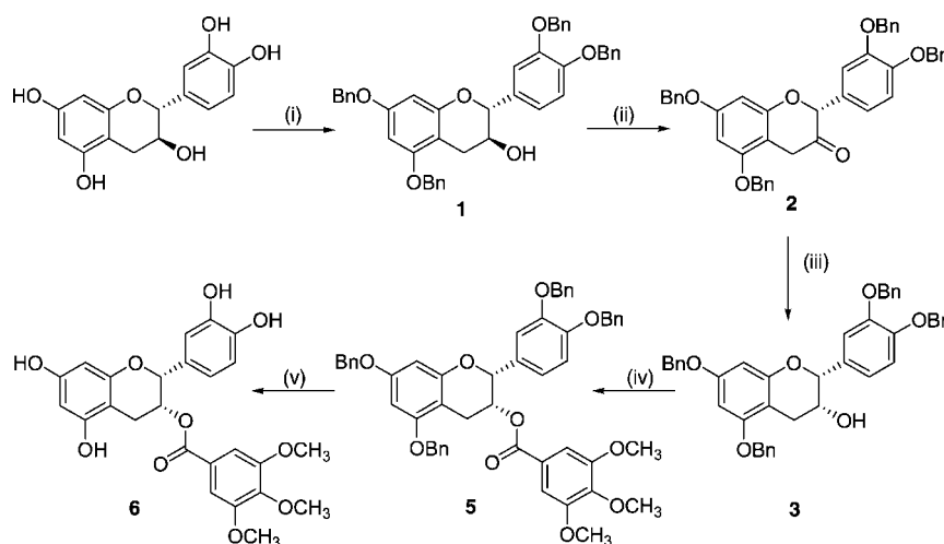
Scheme 1. Synthesis of 3- O -(3,4,5-Trimethoxybenzoyl)-(-)-epicatechin 6 a
