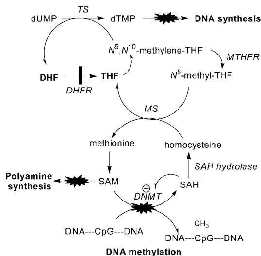
Scheme 2. General Effects of Antifolates on the Folic Acid Cycle a
